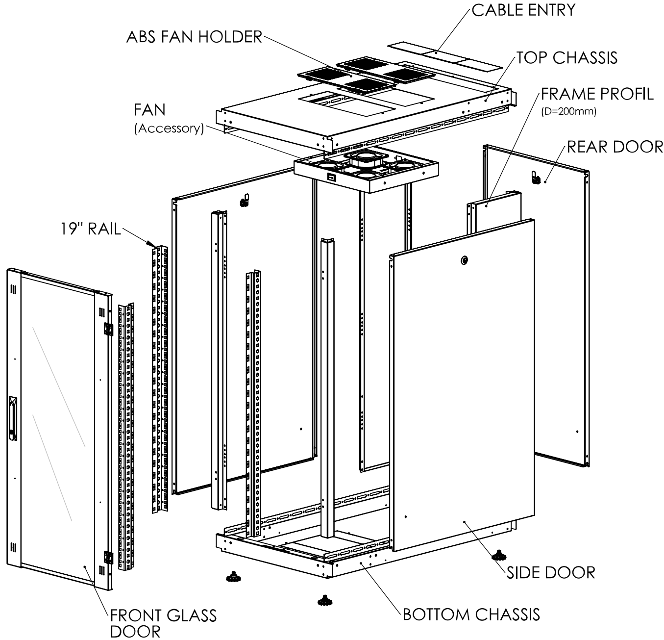
Exploded view
