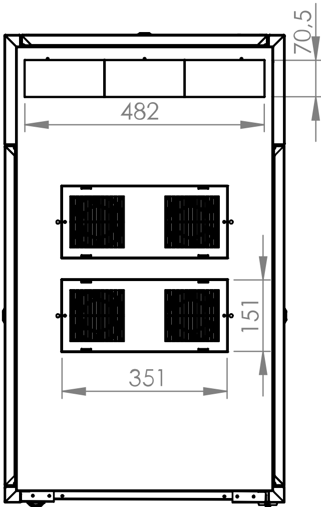
Top view
