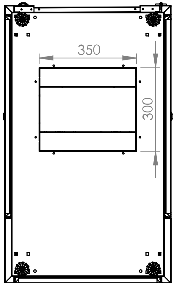
Bottom view
